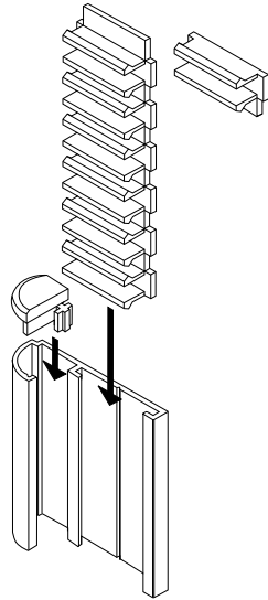
SignBands
